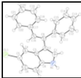
Fig. 1. Molecular structure of the title compound with the atom numbering scheme. Displacement ellipsoids are drawn at the 50% probability level. H atoms are presented as small spheres of arbitrary radius.
