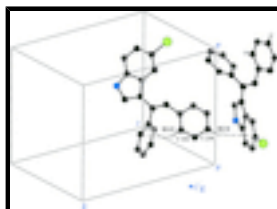
Fig. 2. C—H... \pi interactions (dashed lines) in the title compound. C_g denotes the ring centroid. [Symmetry codes: (i) x, y, z ; (ii) 1 - x, -1/2 + y, 1/2 - z ]
